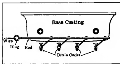
Fig. 3—How cocks may be connected so that they can all be opened at one time
